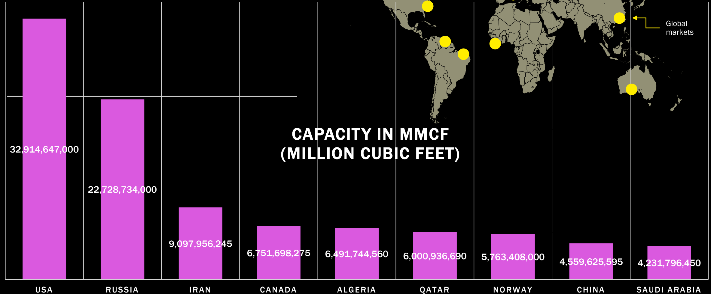
Natural Gas Production by Country
